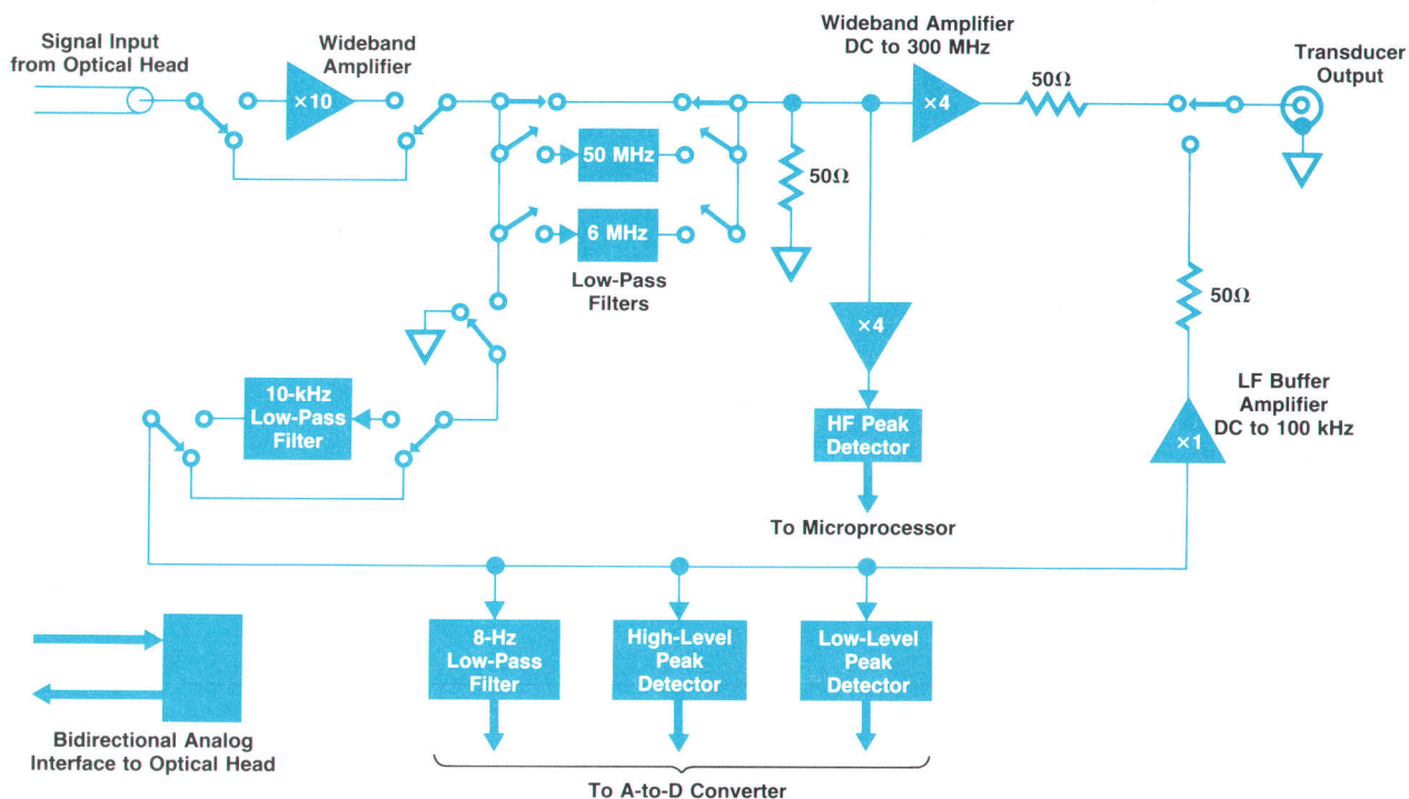
Fig. 6. Like the optical head, the HP 81511A Optical Pulse Power Meter has two paths, a wideband path and a high-sensitivity path. Peak detectors measure the high and low signal levels, and an 8-Hz low-pass filter produces an average signal.
