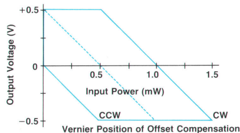
Fig. 2. Offset compensation allows adjustment of the input power that produces a 0V output.
