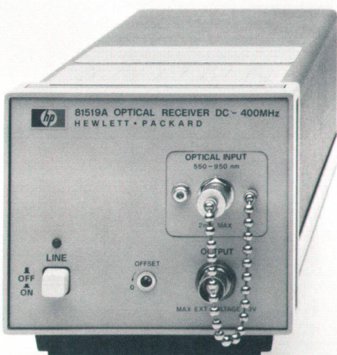
Fig. 1. The HP 81519A Optical Receiver converts optical power to electrical signals with a calibrated conversion factor of -1\text{V/mW} . It operates over an optical wavelength range of 550 nm to 950 nm and has an electrical bandwidth of dc to 400 MHz.
