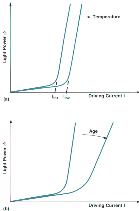
Fig. 7. (a) Temperature dependence of laser diodes. The typical temperature coefficient of the threshold current is 1\%/^{\circ}\text{C} . (b) Aging behavior of laser diodes. With time, the threshold current increases and the differential efficiency decreases.
