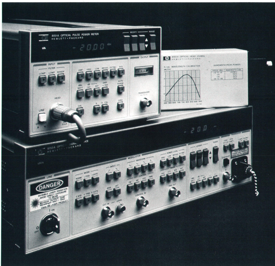
Fig. 1. Two new products, the HP 8150A Optical Signal Source (bottom) and the HP 8151A Optical Pulse Power Meter (top left, shown with the HP 8151A Optical Head), are precise, fully programmable stimulus and response-measuring instruments for design and production testing of fiber optic devices and systems at short wavelengths.
