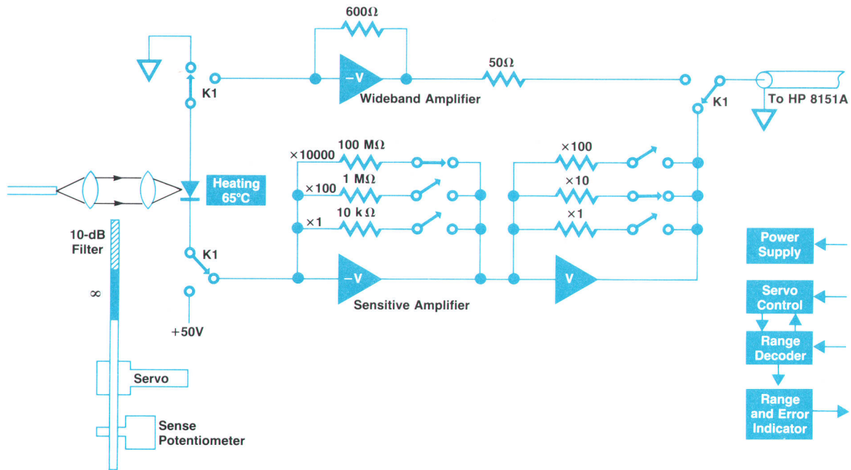
Fig. 3. The HP 81511A Optical Head has a wideband, dc-to-250-MHz path for optical power between -10 dBm and +10 dBm, and a very sensitive, narrowband, dc-to-4-kHz path for optical power down to -60 dBm.
