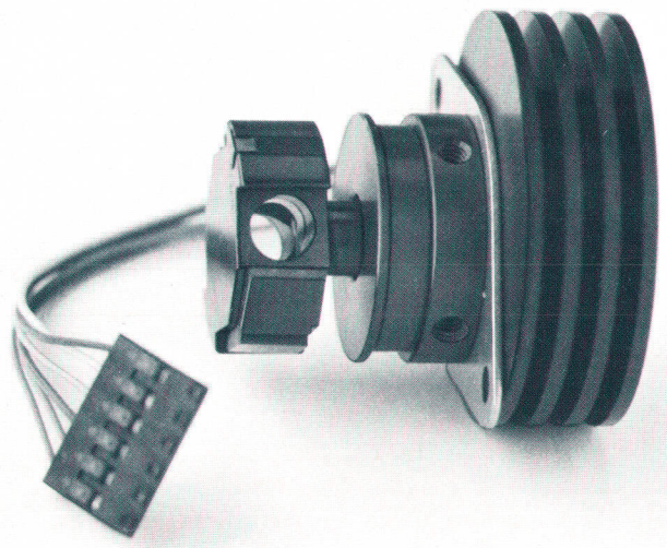
Fig. 18. Step attenuator assembly (0, 20, or 40 dB or \infty ).
