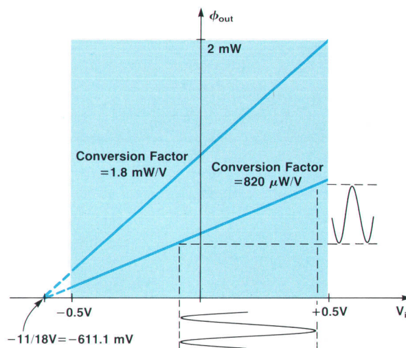
Fig. 4. With external modulation, the user can select the conversion factor in milliwatts, microwatts, or nanowatts of optical output per volt of electrical input.
