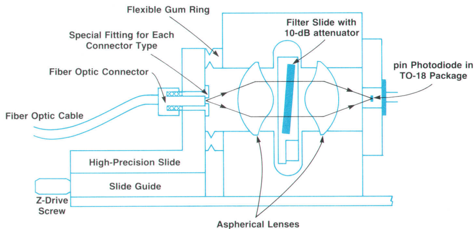
Fig. 5. The HP 81511A Optical Head accommodates different types of fiber optic connectors by using a special fitting for each connector type. The slide carrying the fitting is adjustable with respect to the focal point of the lens system inside the head.
