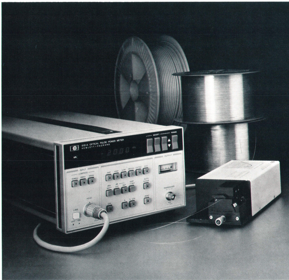
Fig. 1. The HP 8151A Optical Pulse Power Meter (left) measures and displays peak and average optical input power levels. It has a bandwidth of dc to 250 MHz for optical power between -20 dBm and +10 dBm. Its optical-to-electrical transducer is in a separate optical head (right) connected by a cable to the mainframe.
